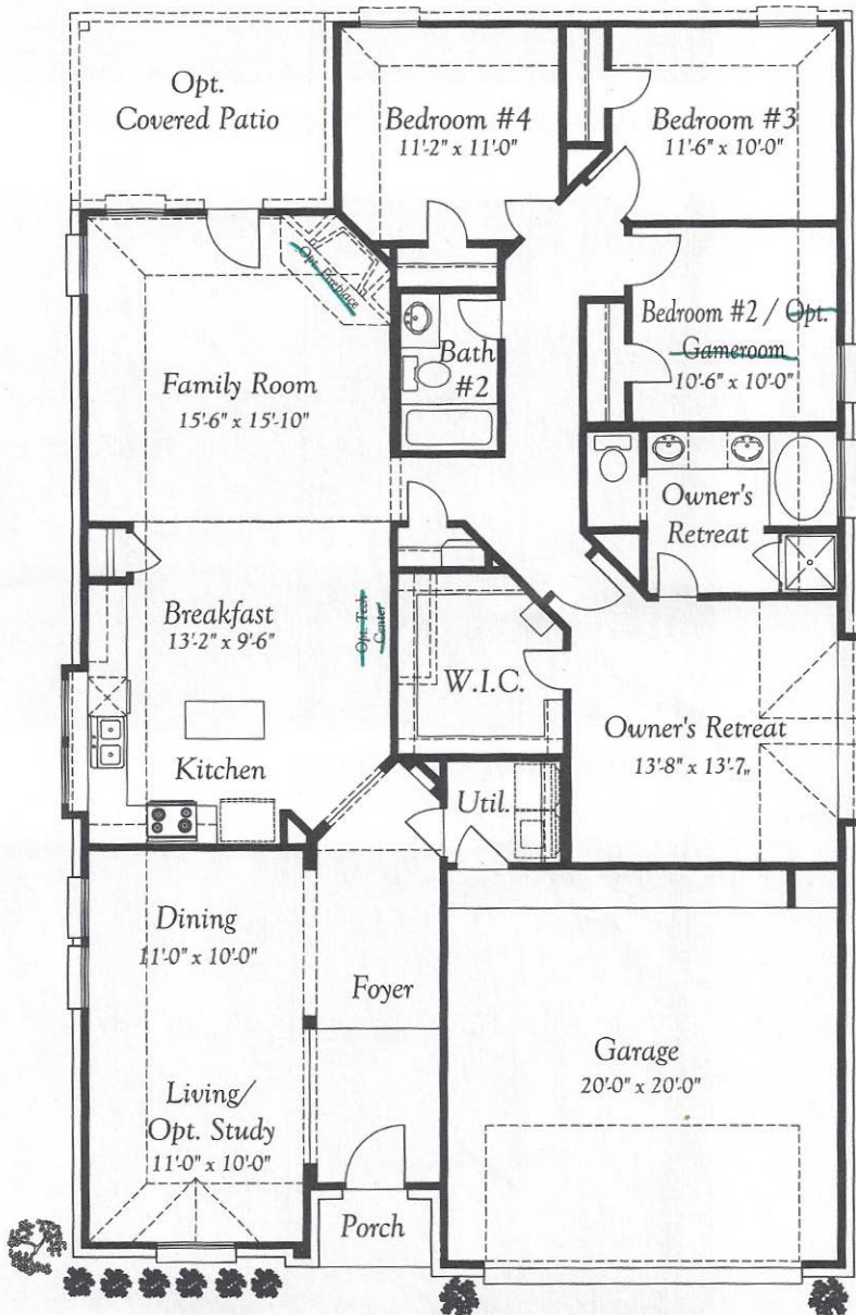
FLOORPLAN
