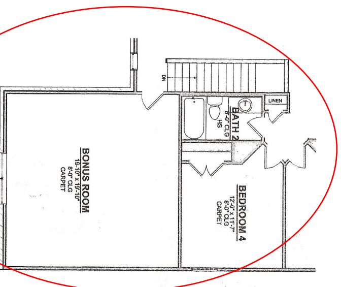
Second Floor Plan w/ Opt. Bonus Room
