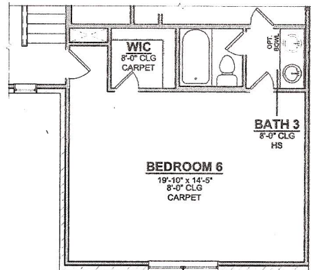
Opt. Bedroom 6/ Bath 3 ILO Opt. Bonus Room
