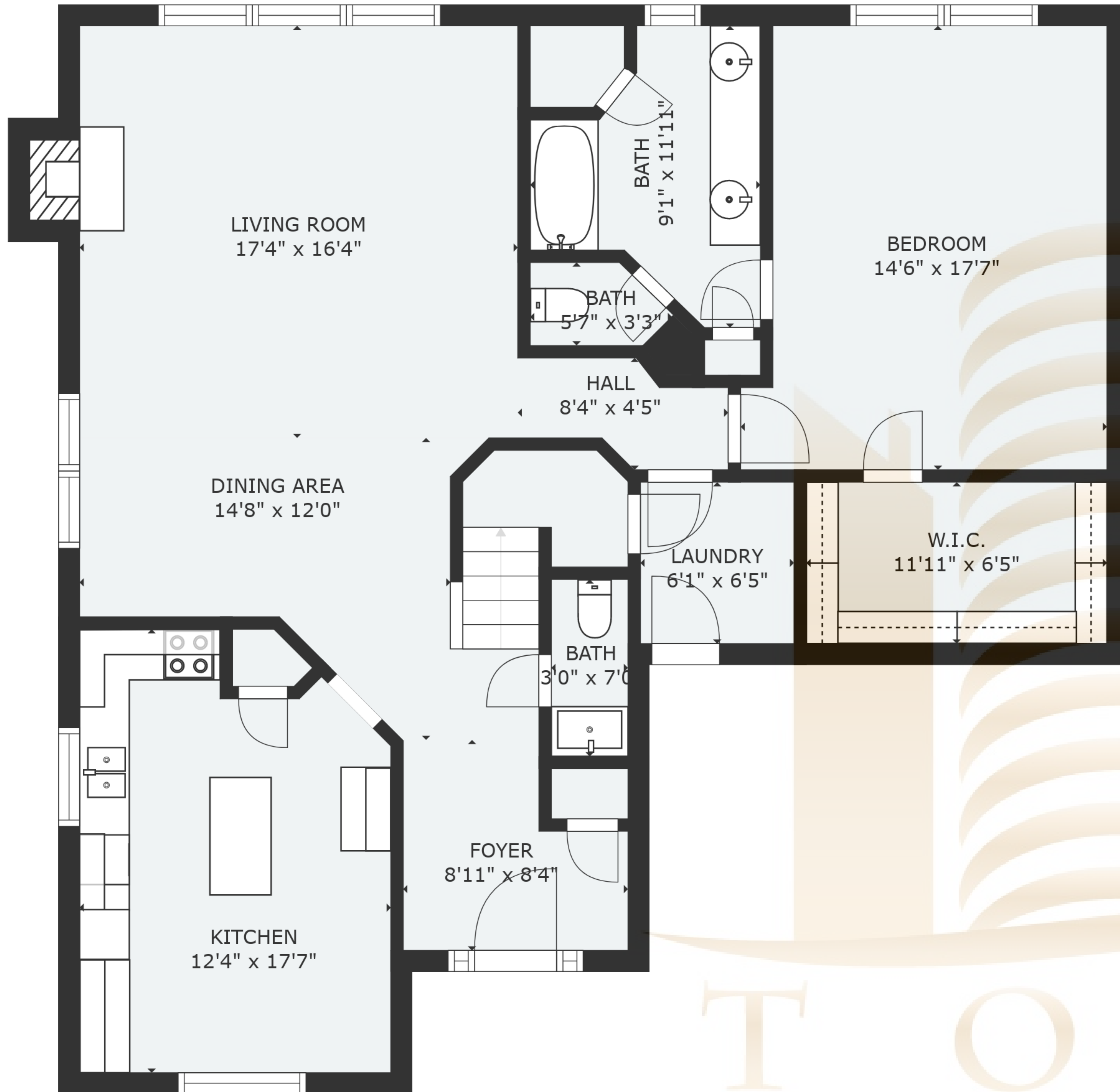
FLOOR 1
