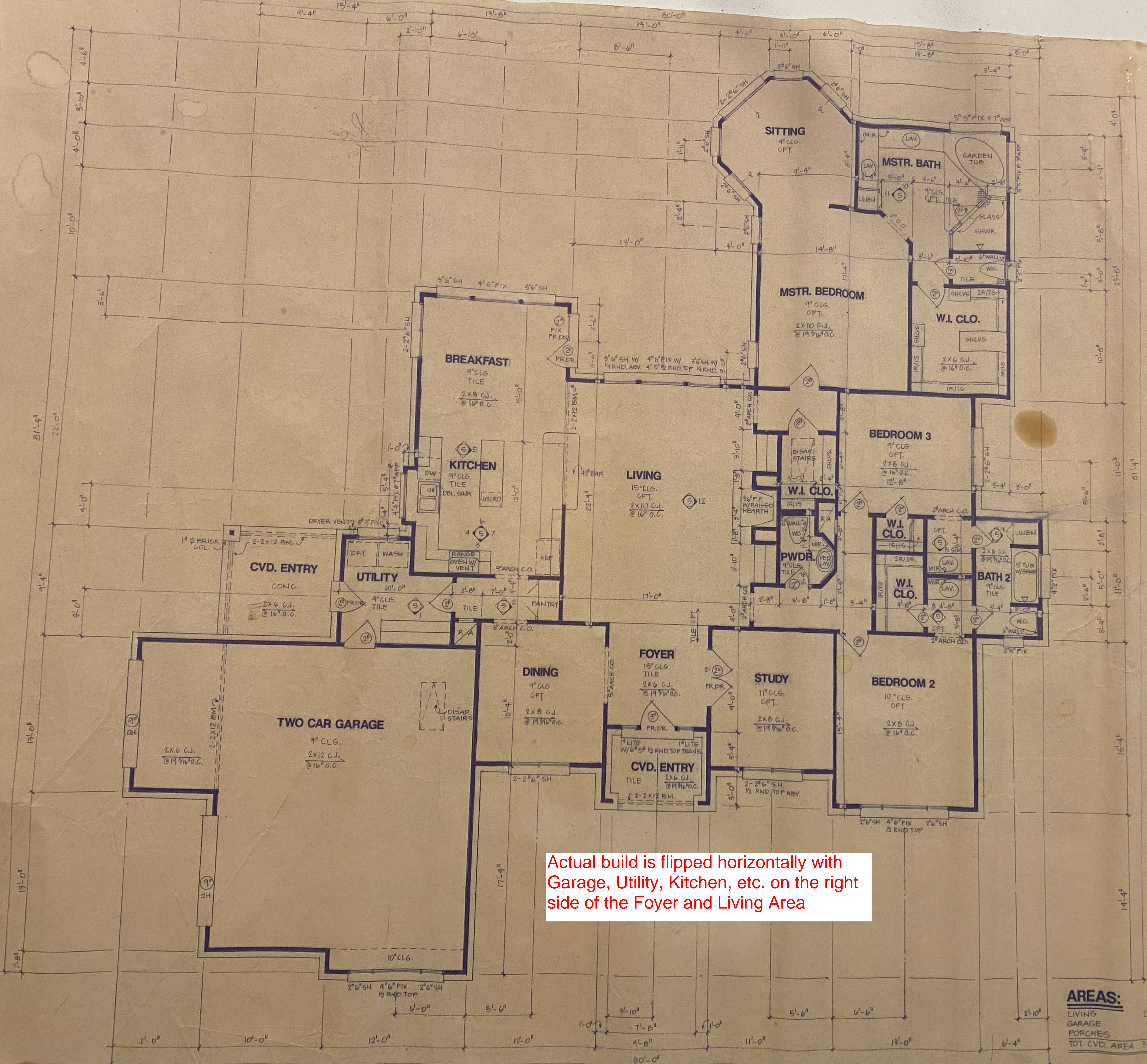
FLOOR PLAN 1/4"
