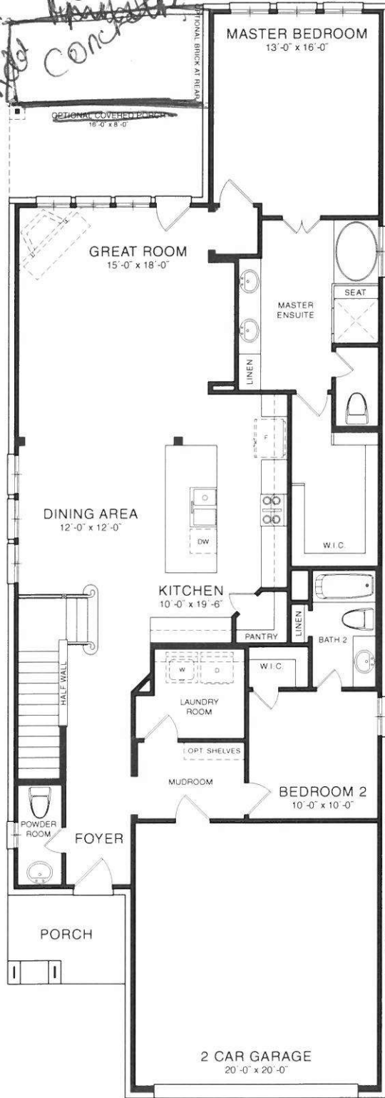
MAIN FLOOR PLAN STYLE A
