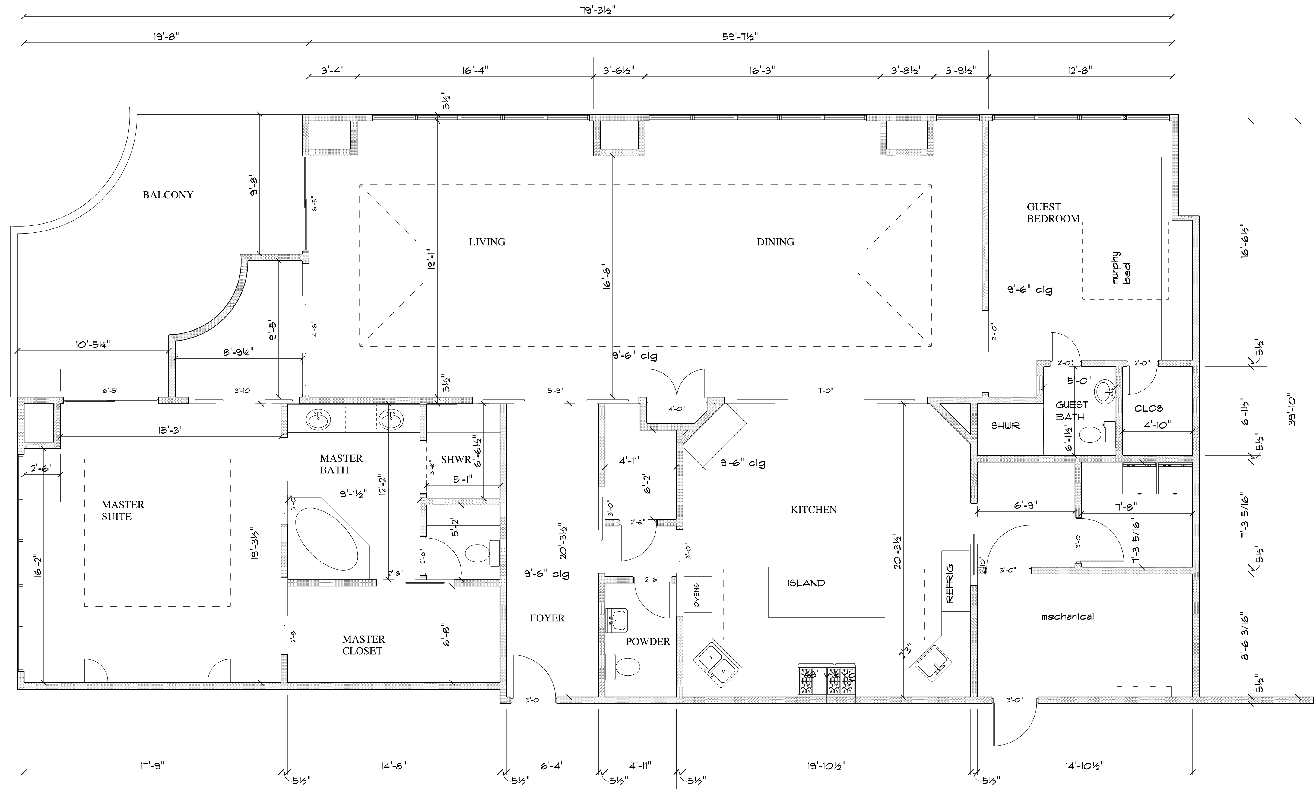
FLOOR PLAN 2121 KIRBY DRIVE #10 SW HUNTINGTON HOUSTON TX
