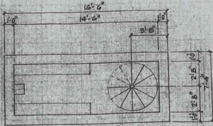
CELLER PLAN
