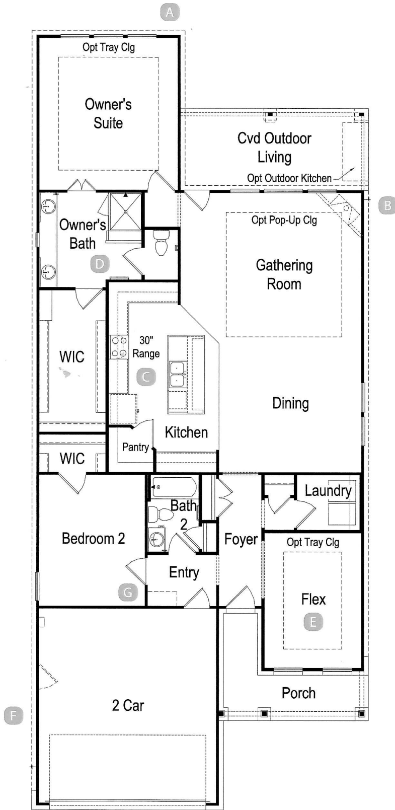
FIRST FLOOR
