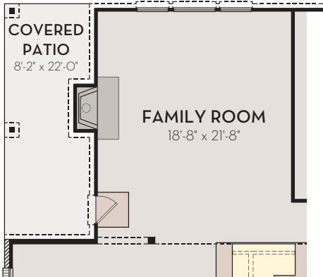
OPT. EXTENDED FAMILY ROOM 85 SQ. FT.
