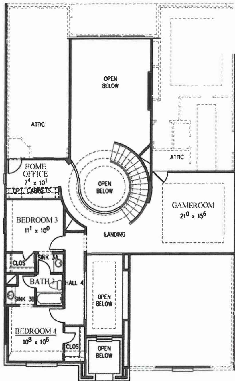
SECOND FLOOR
