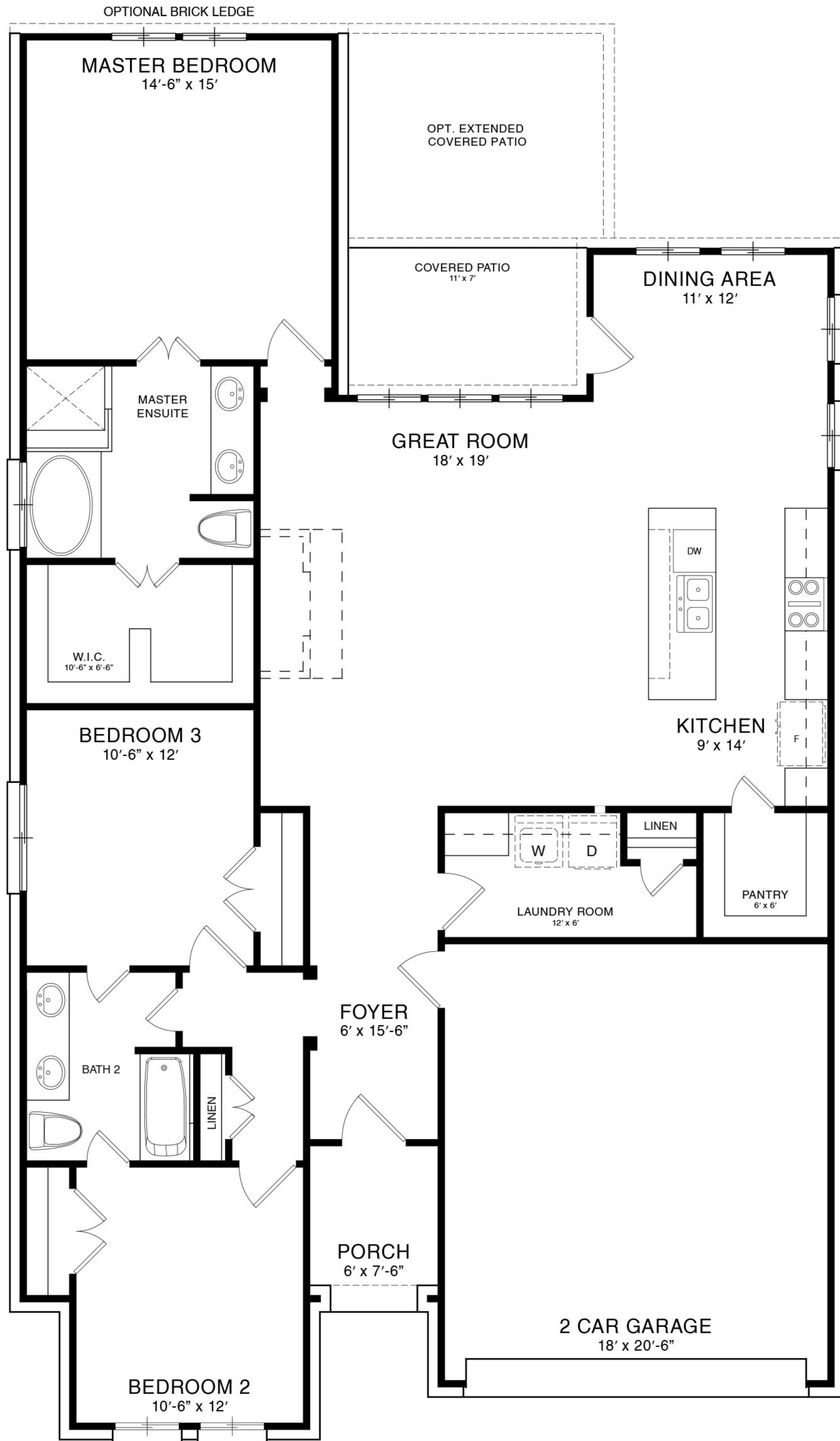
MAIN FLOOR PLAN STYLE A
