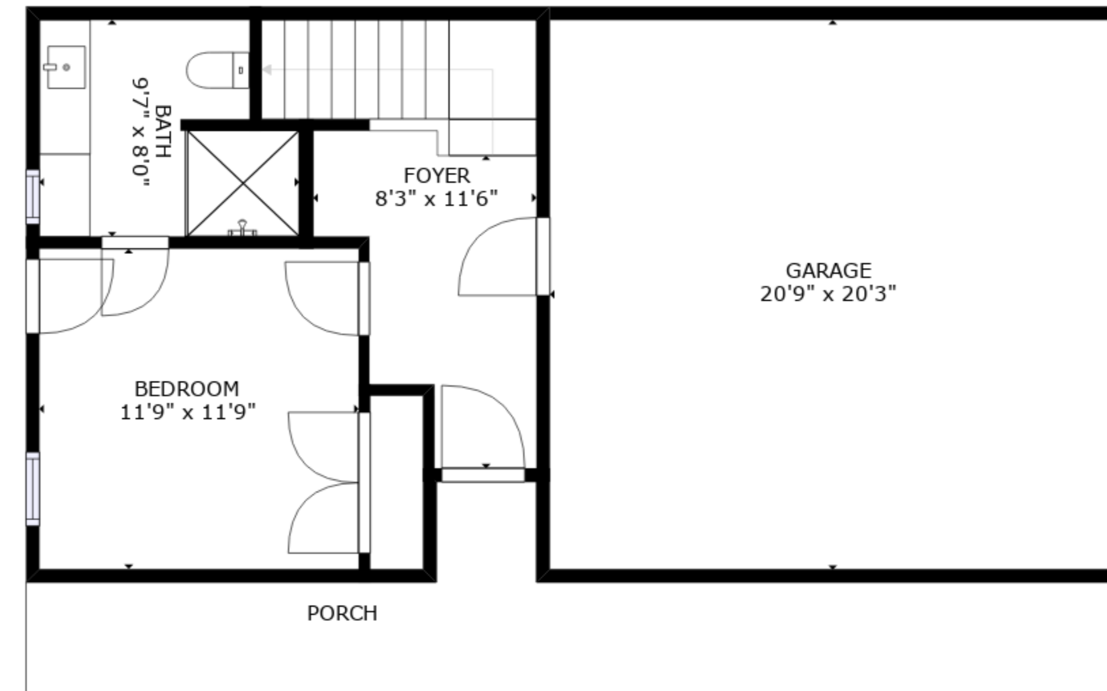
FLOOR 1
