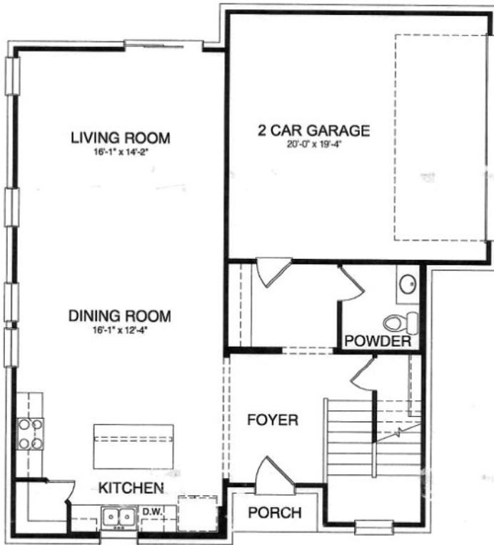
MAIN FLOOR PLAN ELEVATION A
