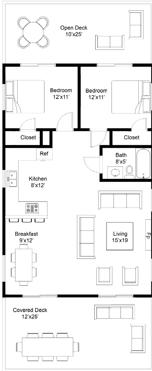
FLOOR PLAN
