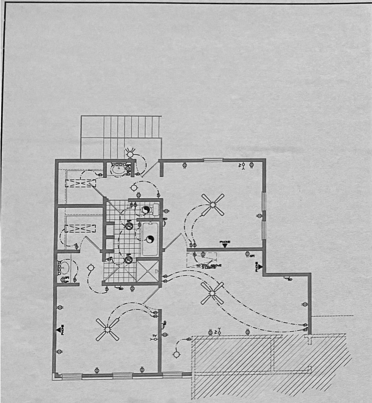
ELECTRICAL PLAN
