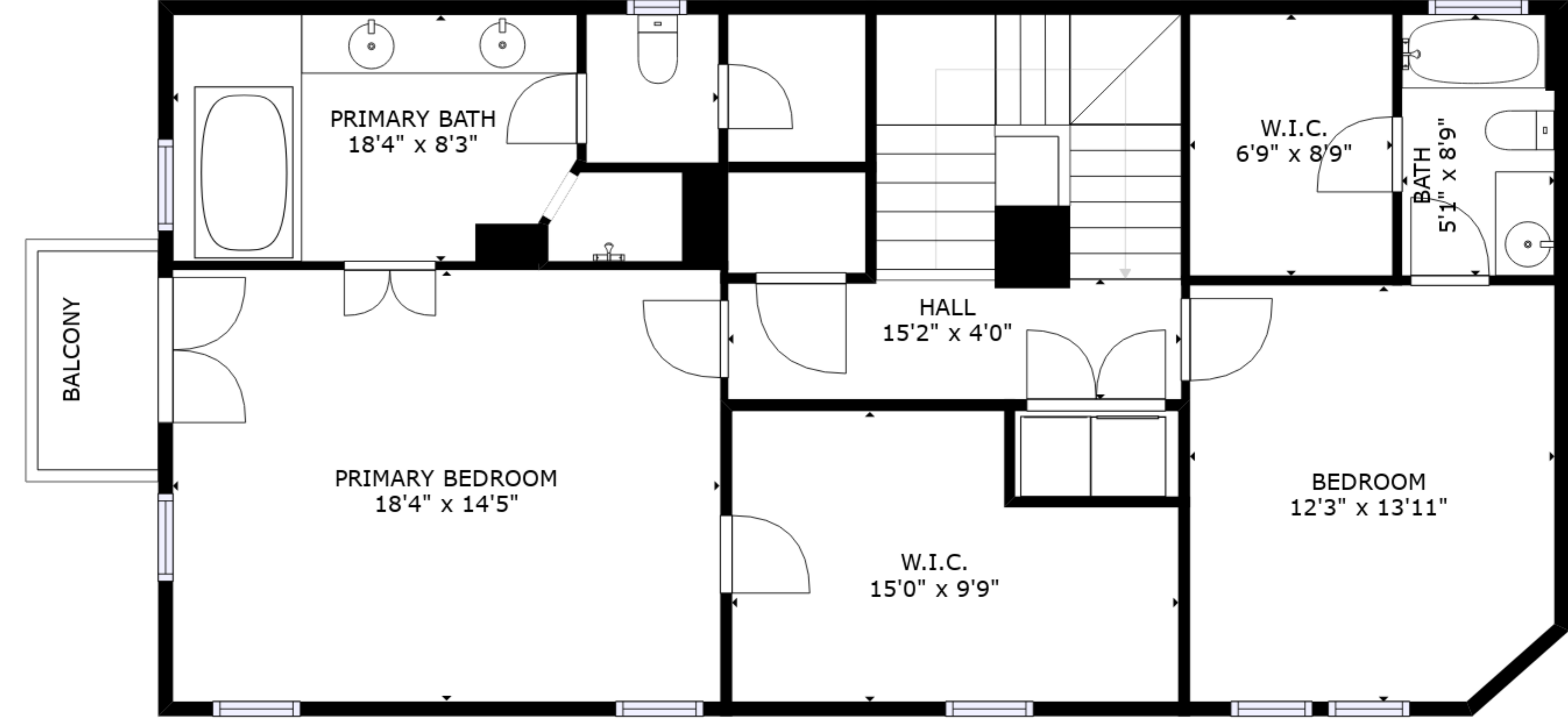
FLOOR 3
