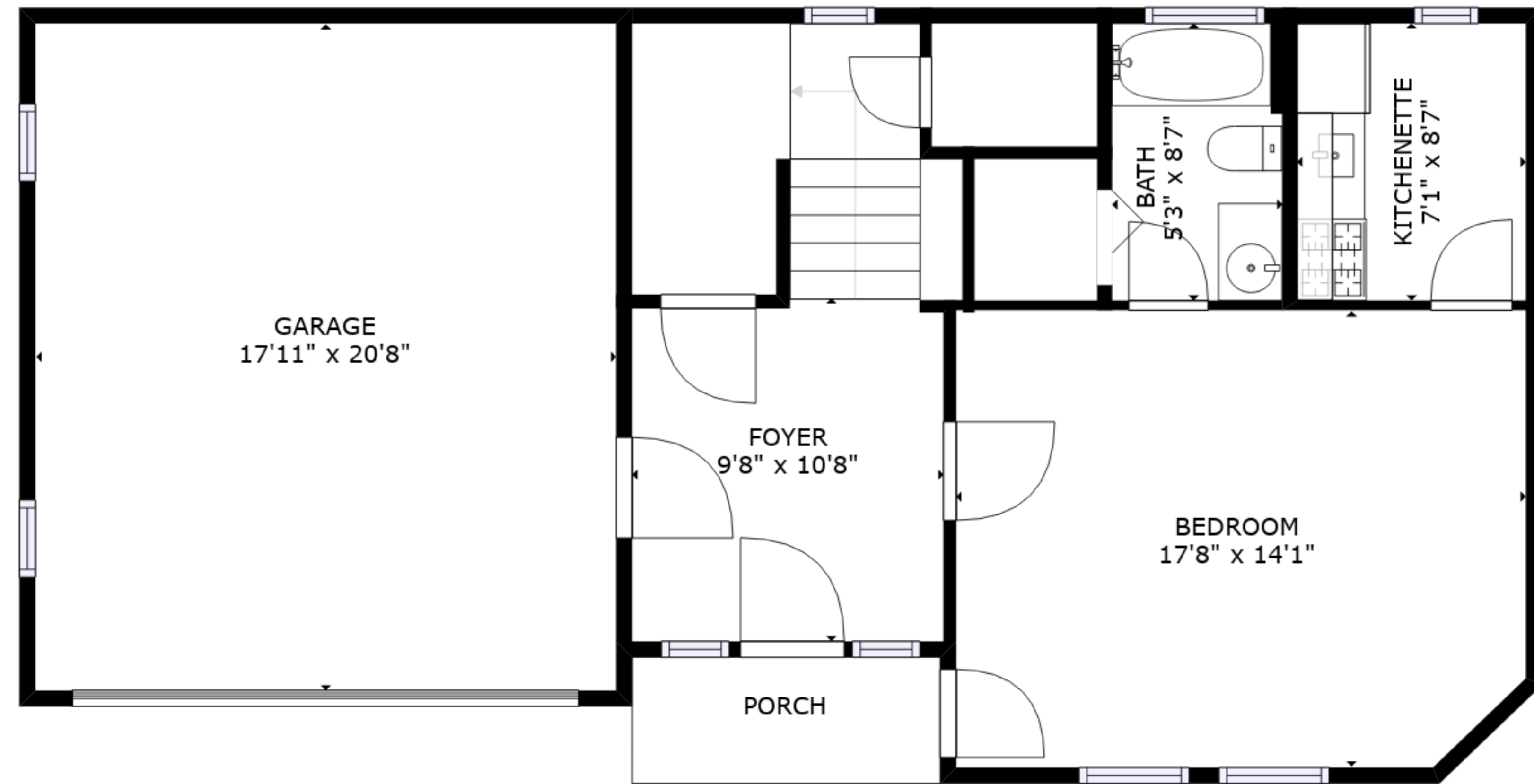
FLOOR 1
