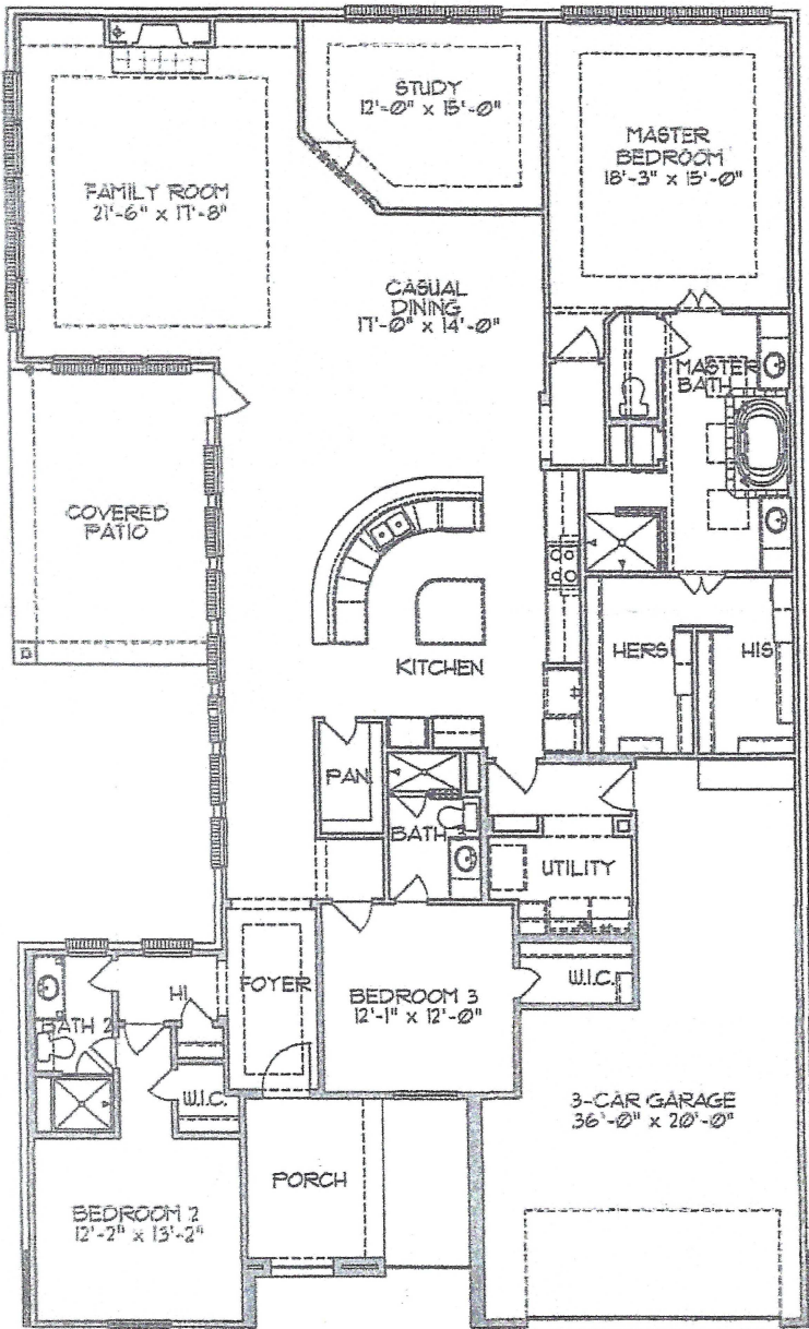
FLOOR PLAN
