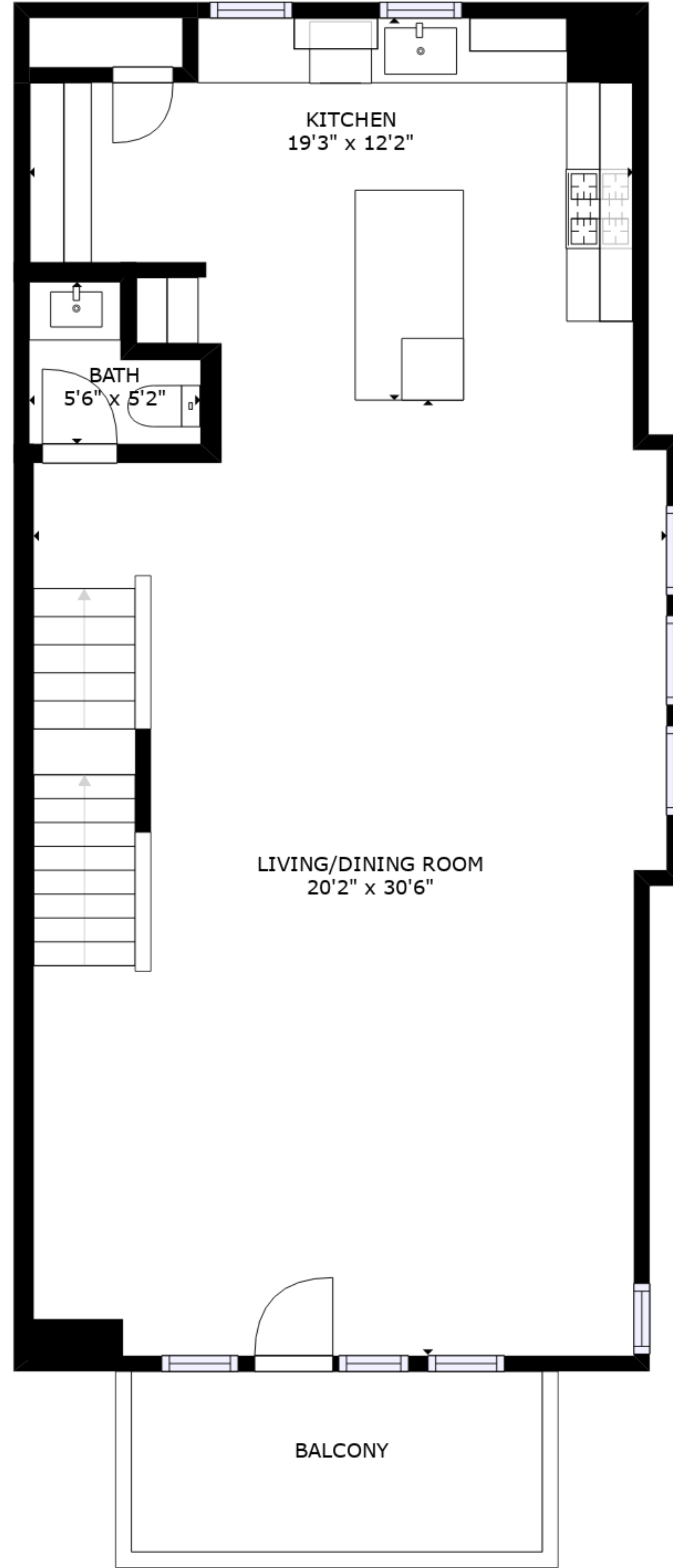
FLOOR 2
