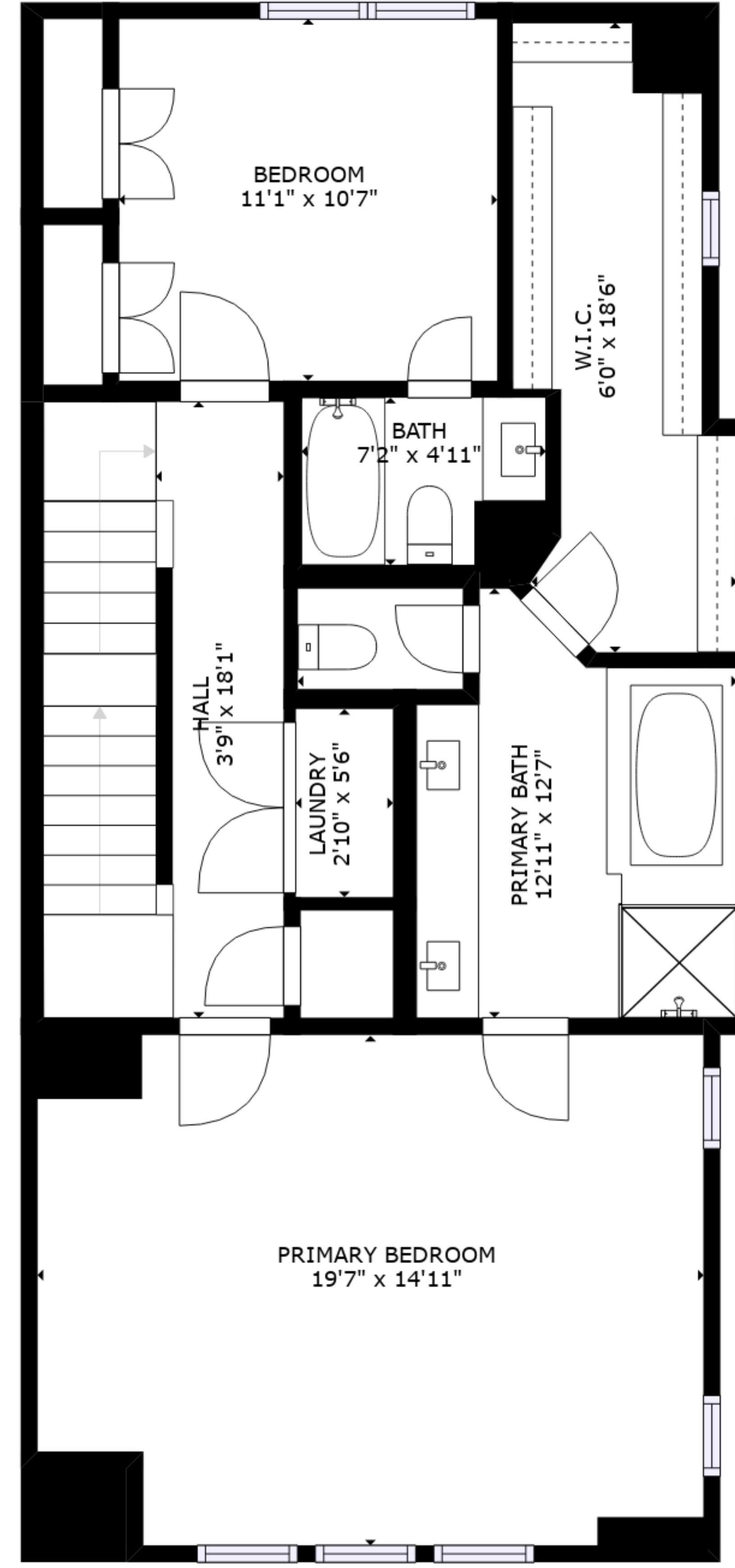
FLOOR 3
