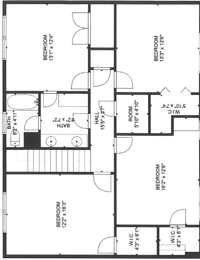
FLOOR 2
