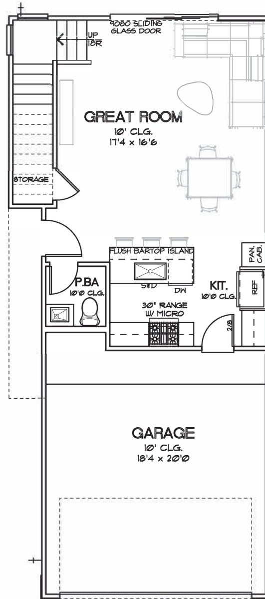
FIRST LEVEL PLAN
