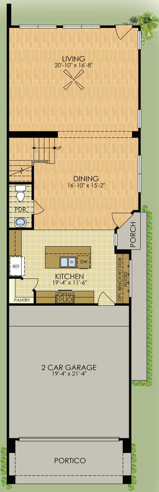
FIRST FLOOR
