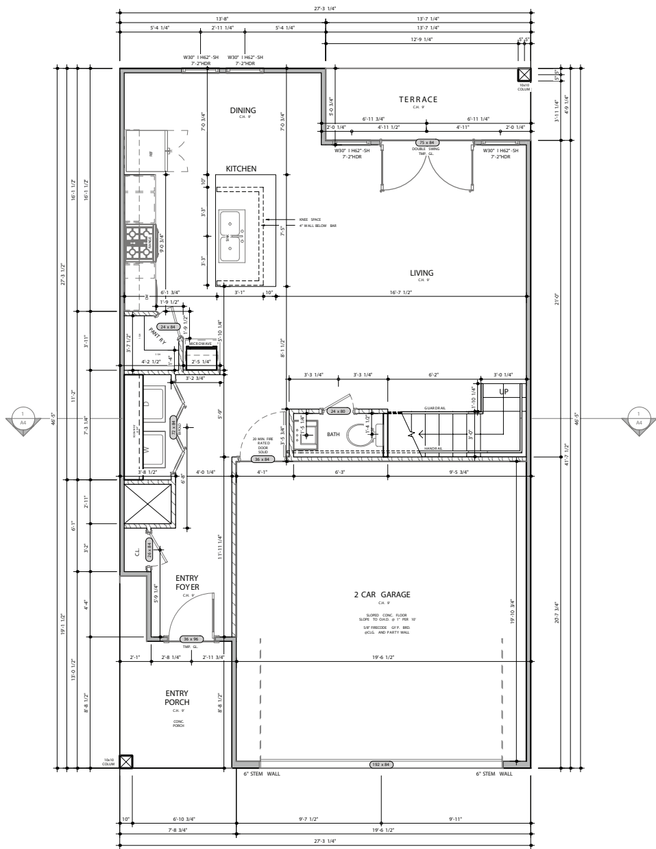
① F.I.N. FLR 1 1/4" = 1'-0"
