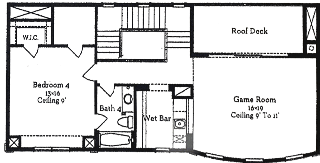
Fourth Floor 875 Sq.Ft
