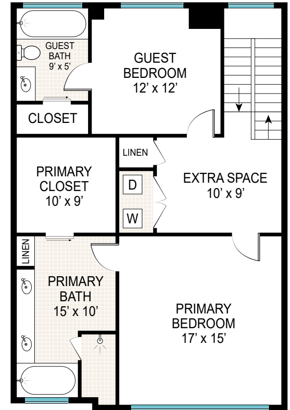
THIRD FLOOR
