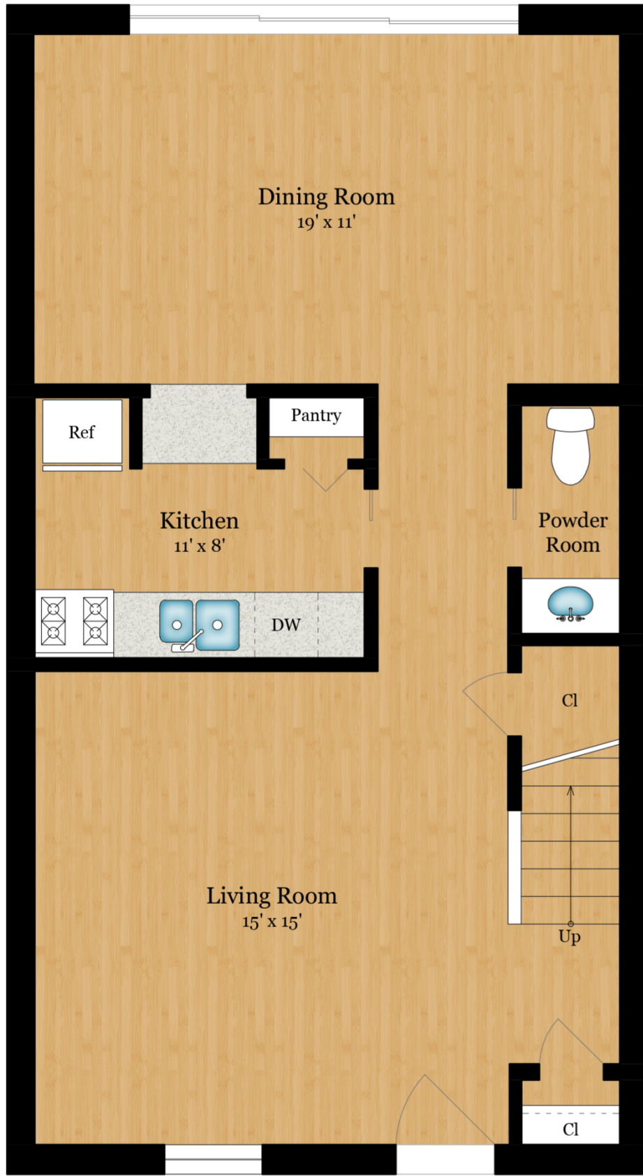
FIRST FLOOR 717 SQ FT
