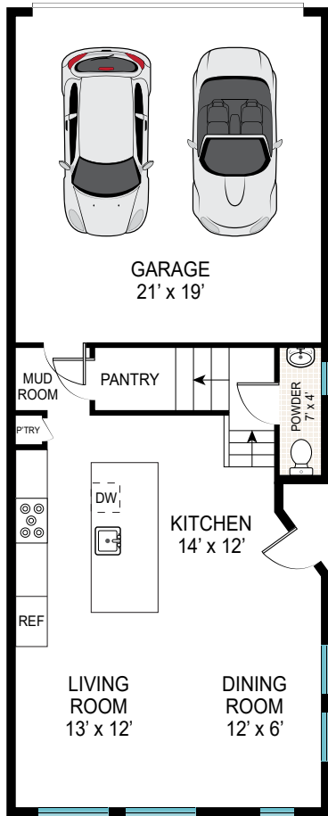
FIRST FLOOR
