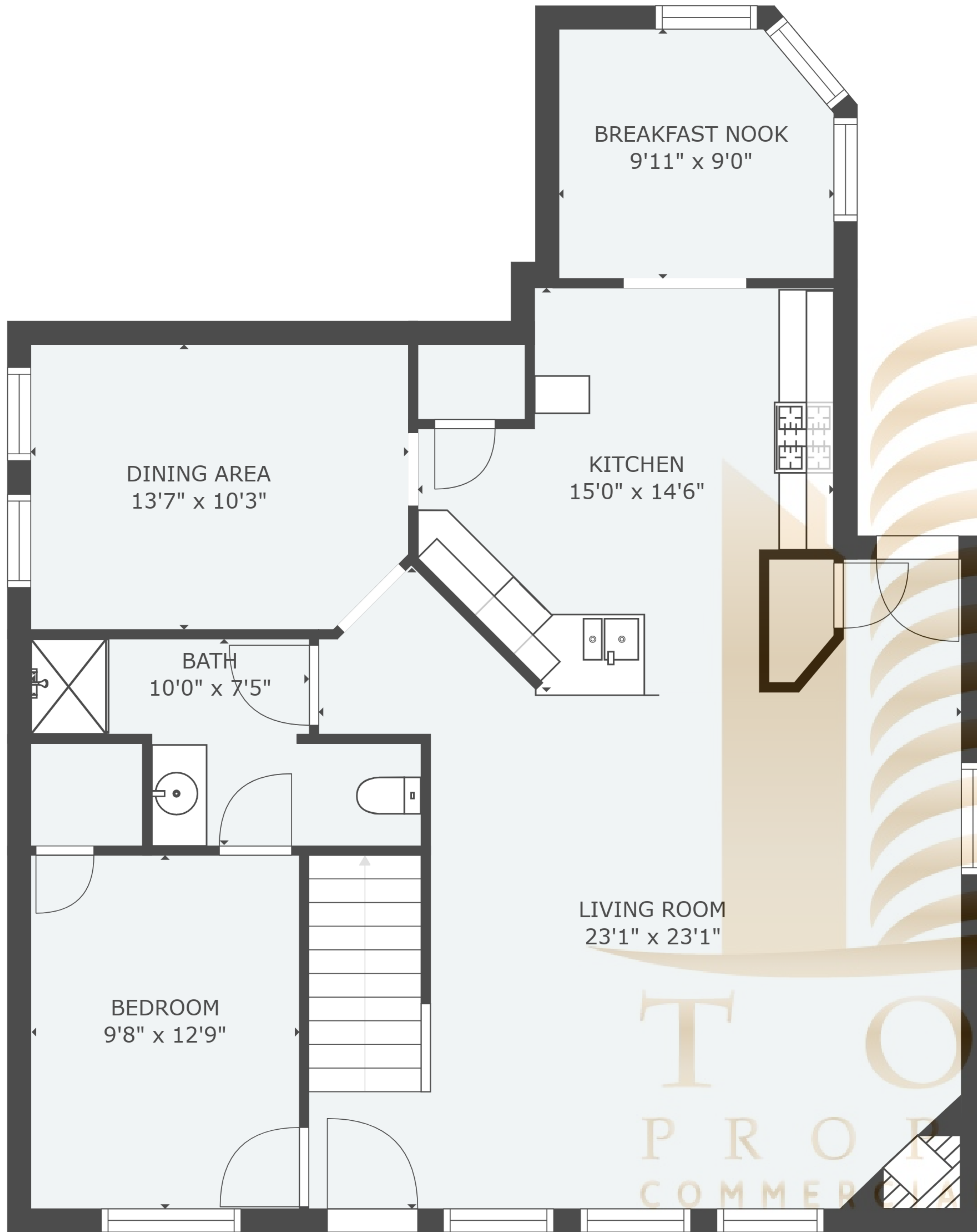
FLOOR 1
