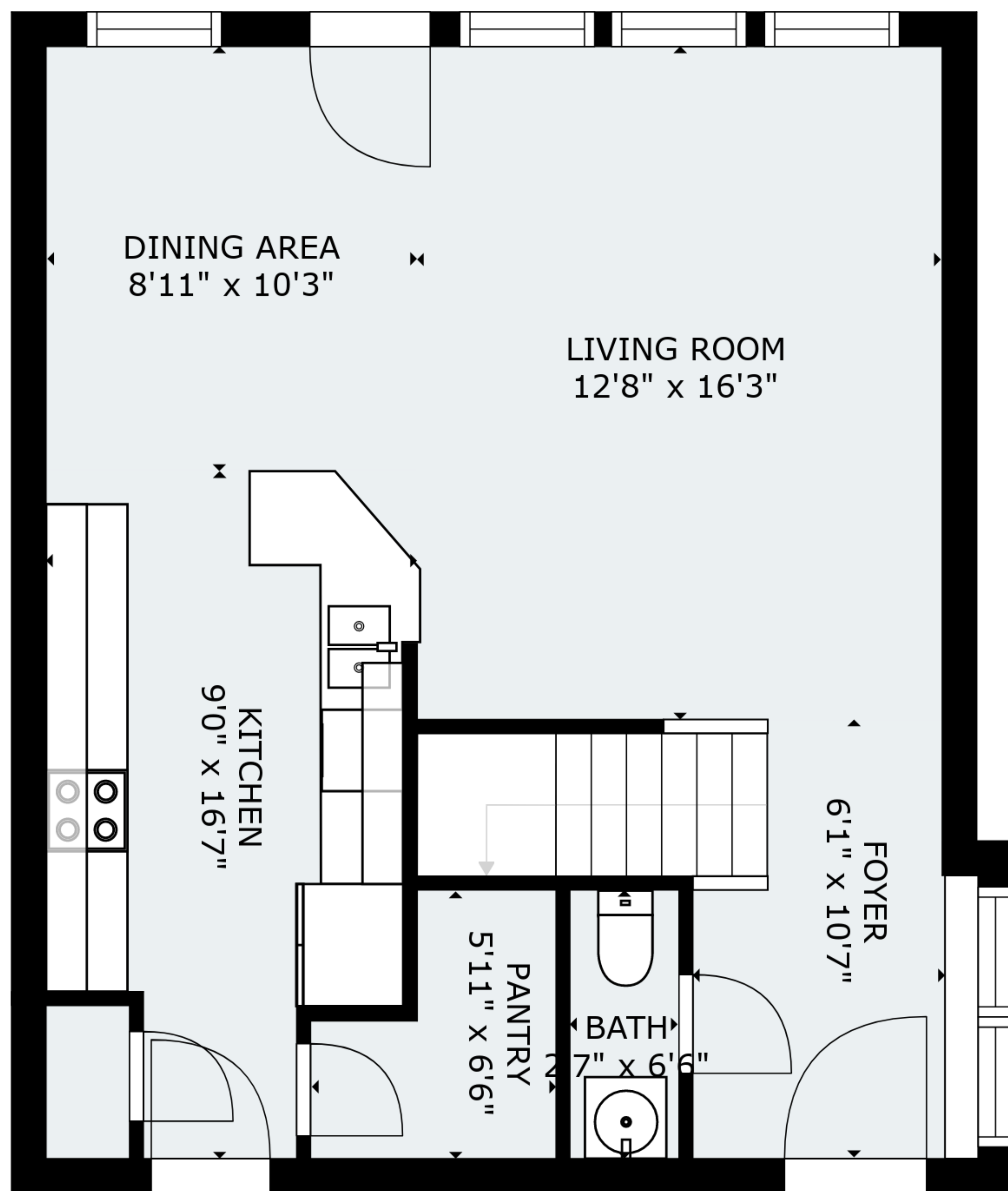
FLOOR 1
