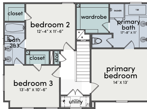
SECOND FLOOR
