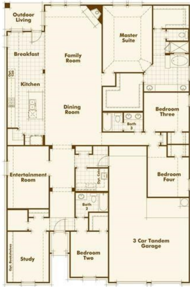
Plan 204 Lower level
