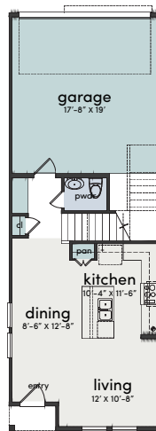
FIRST FLOOR
