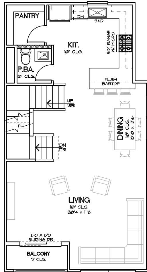
SECOND FLOOR PLAN PLAN 1853 R
