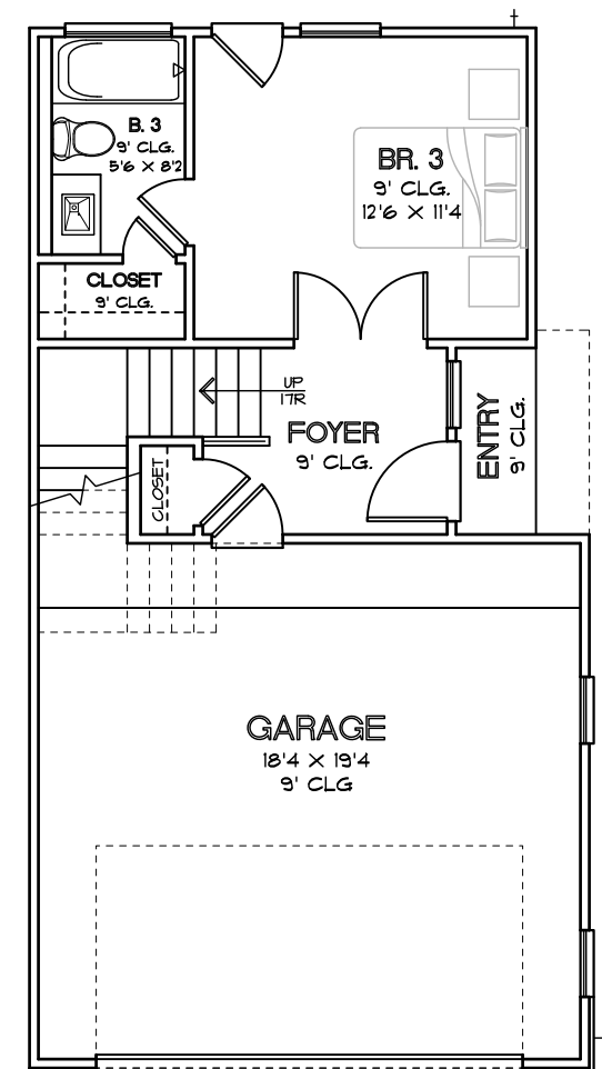
FIRST FLOOR PLAN PLAN 1853 R
