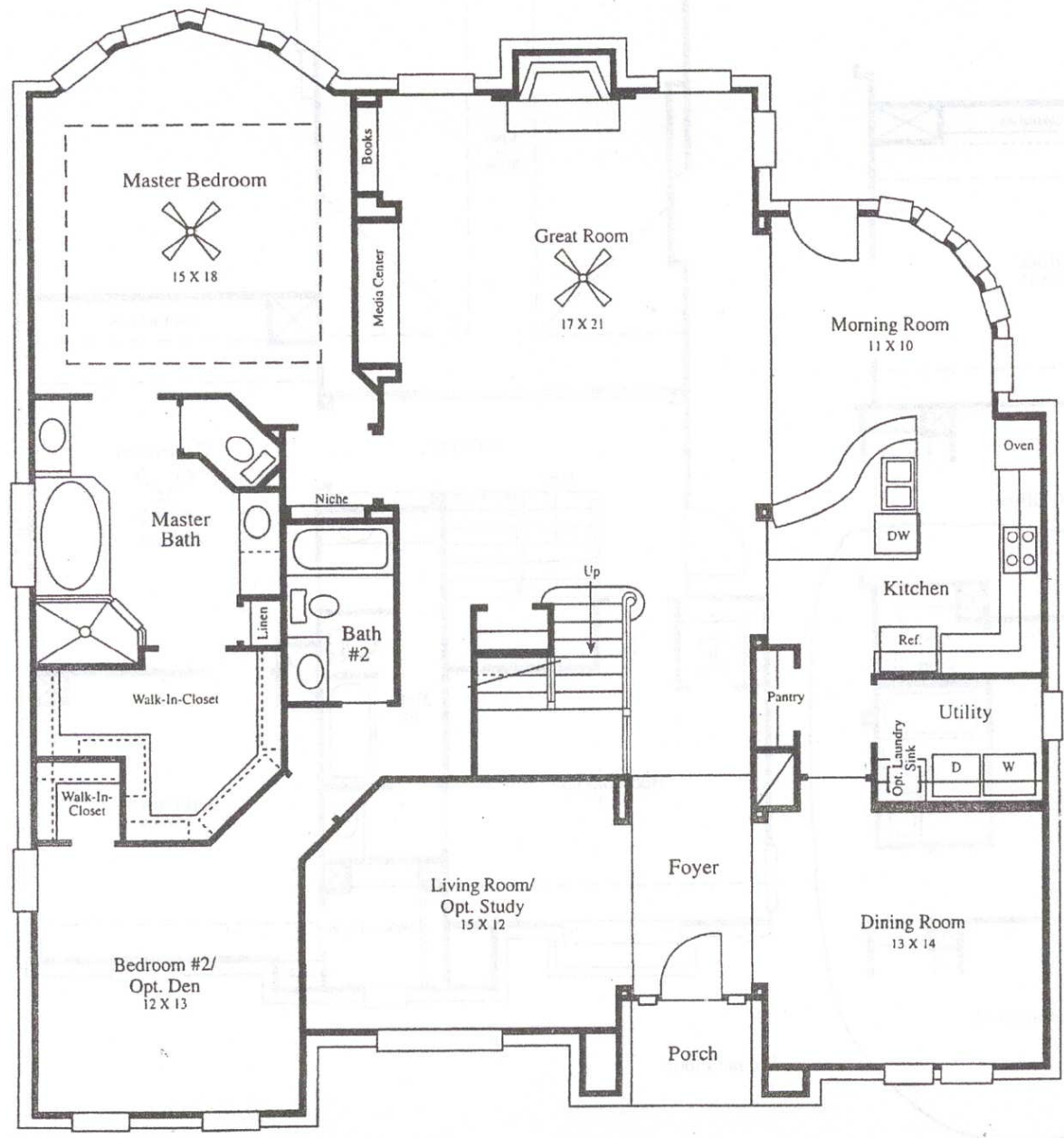
First Floor
