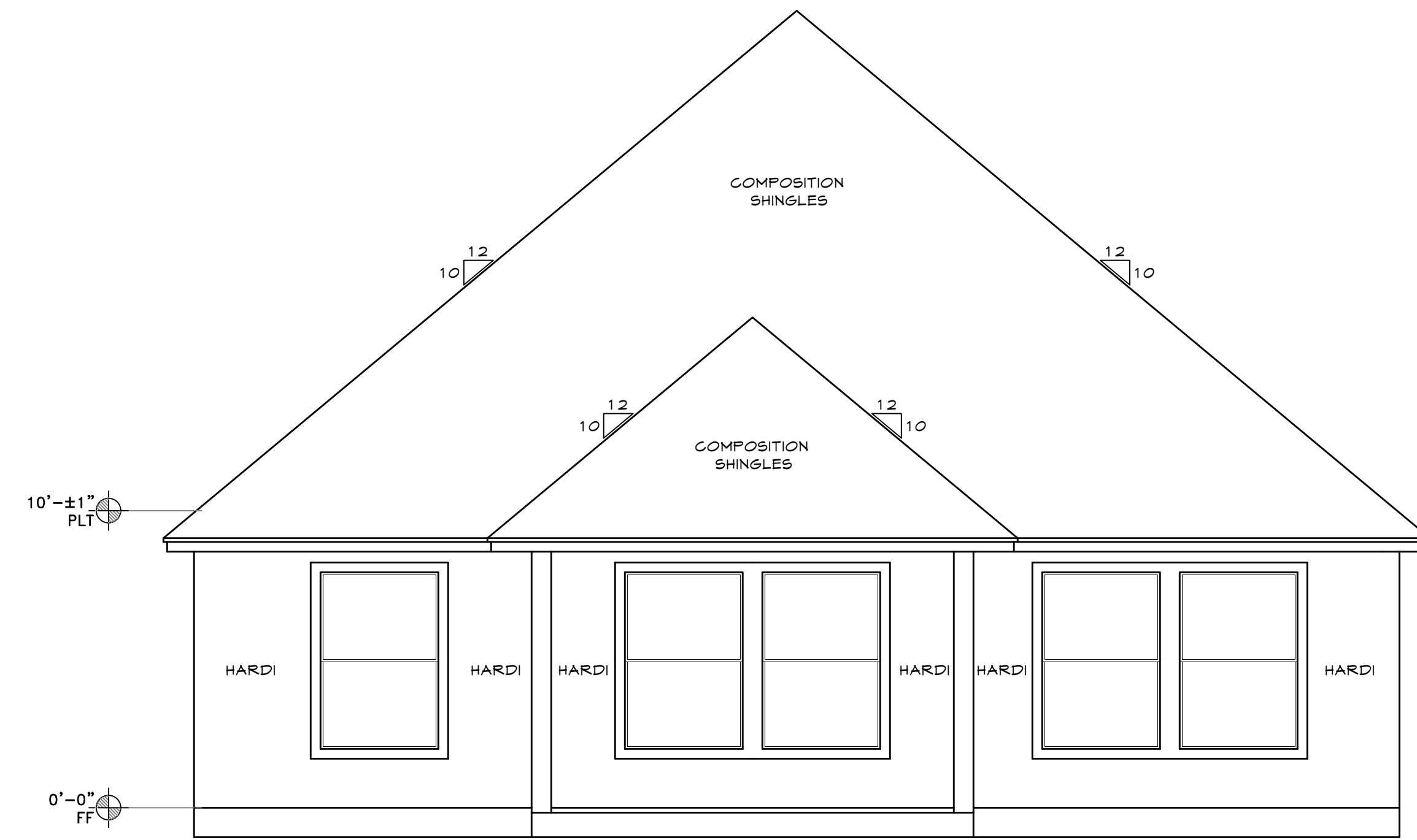
1 REAR VIEW A2 SCALE: 1/4" = 1'
