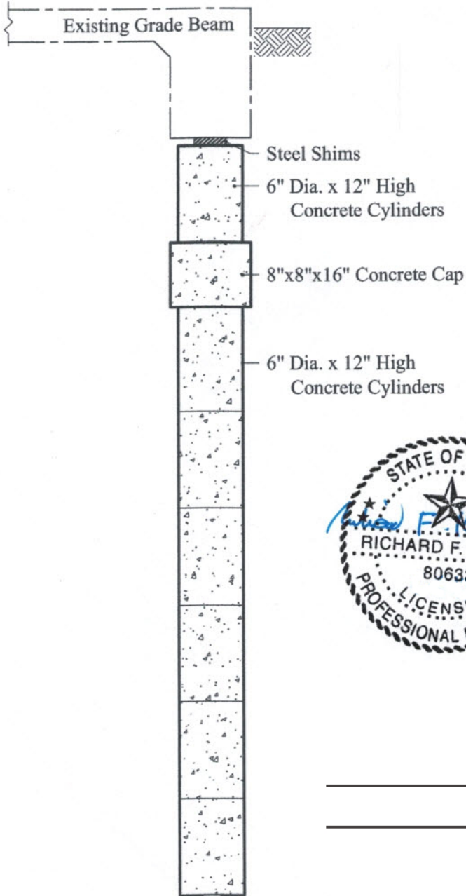
Cutaway View
