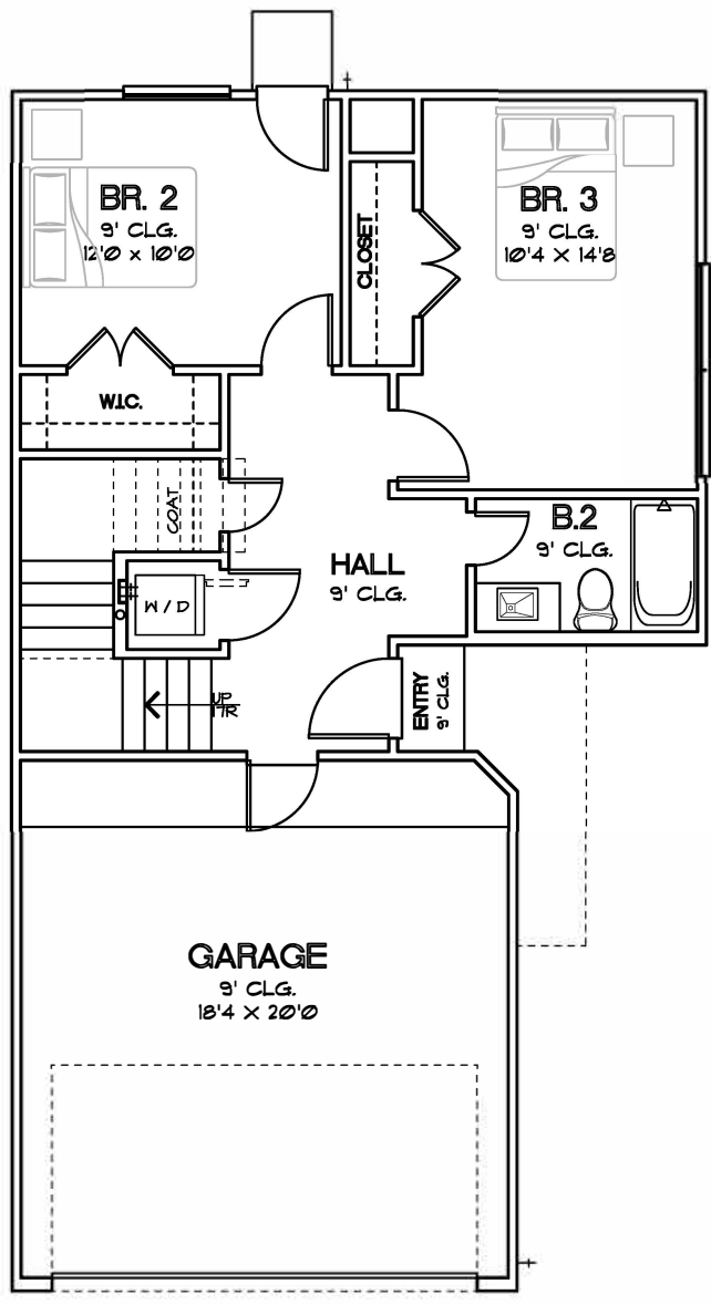
FIRST LEVEL PLAN 1,486 SF
