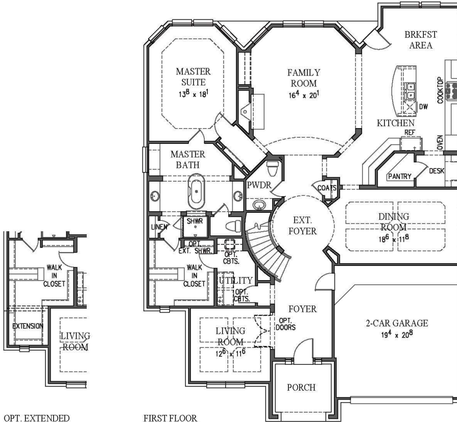
OPT. EXTENDED MASTER CLOSET
