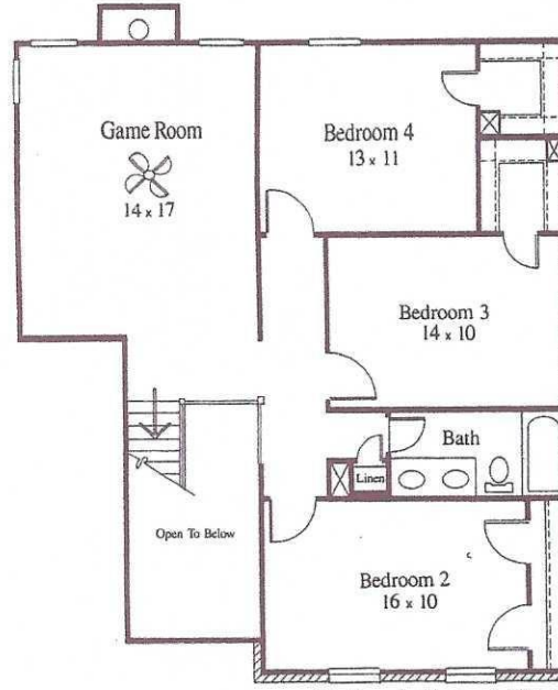
Optional Second Floor
