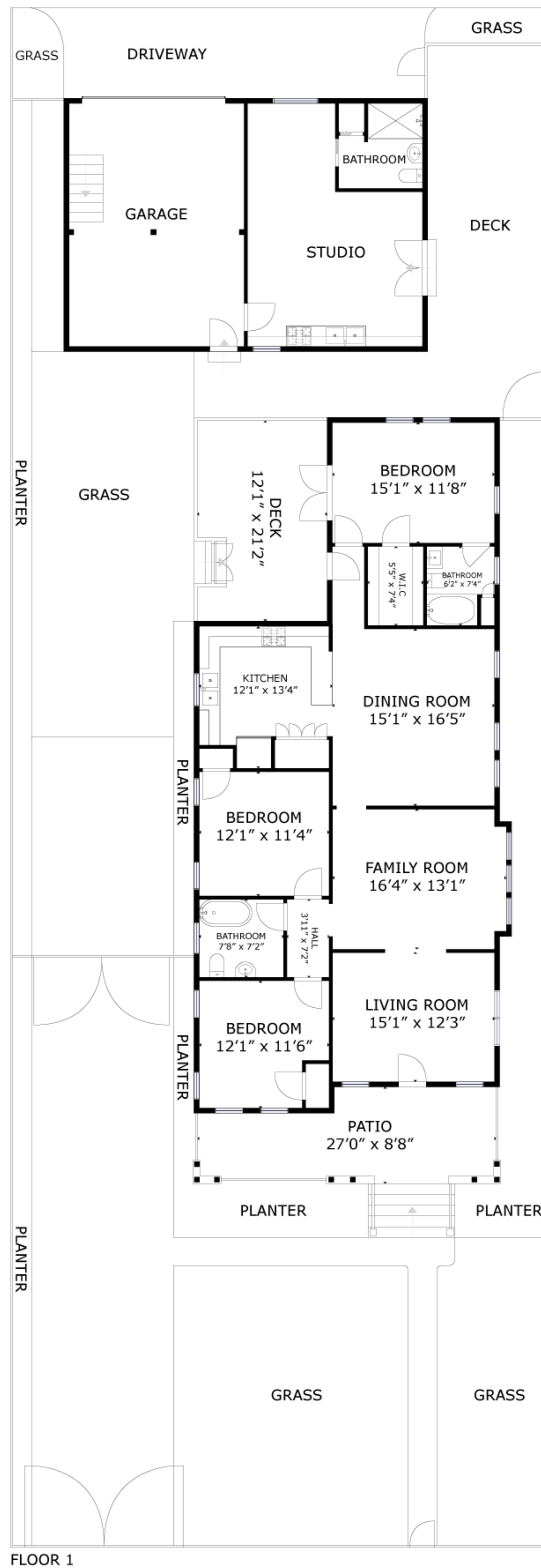
FLOOR 1
