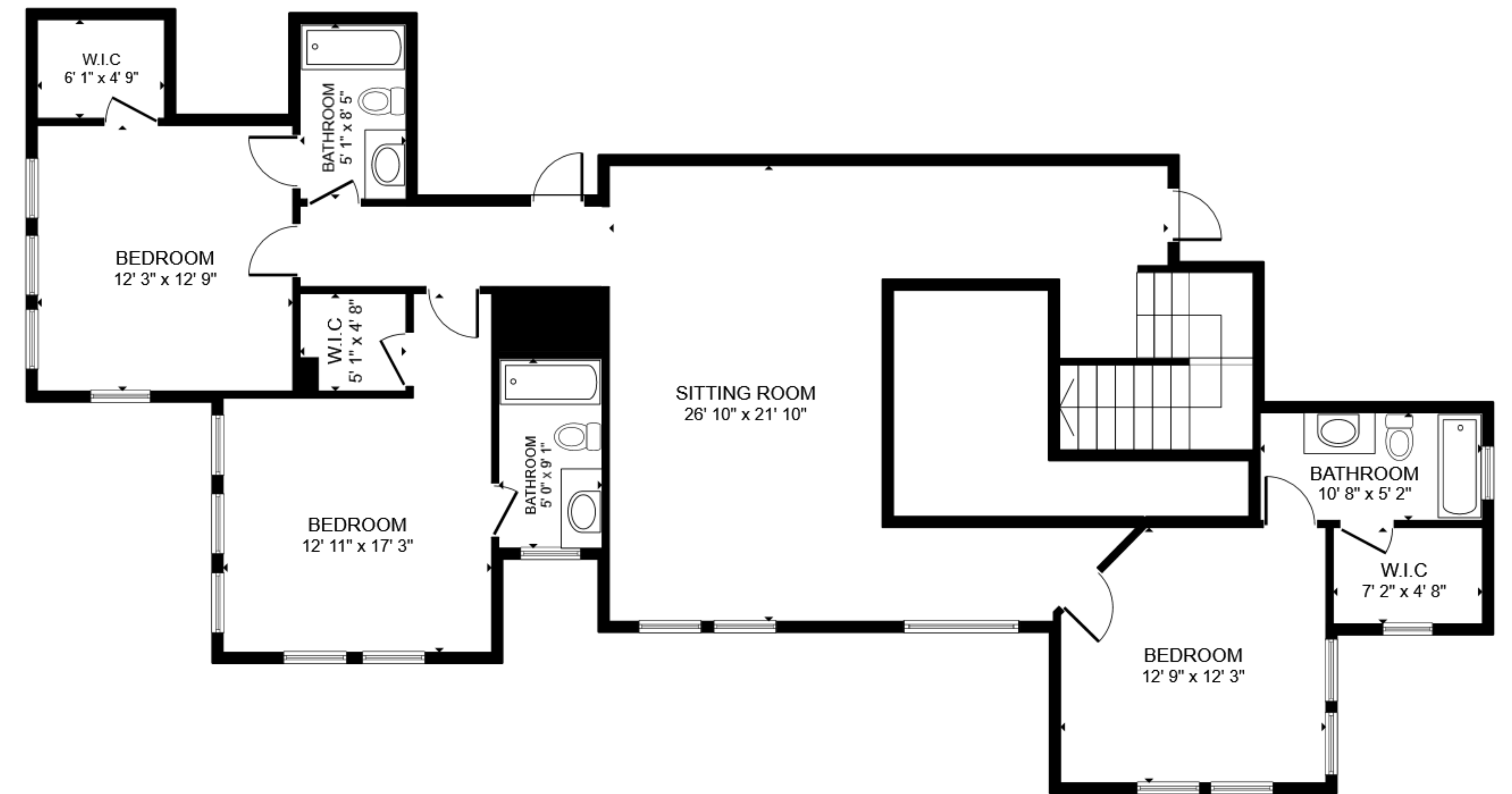
FLOOR 2
