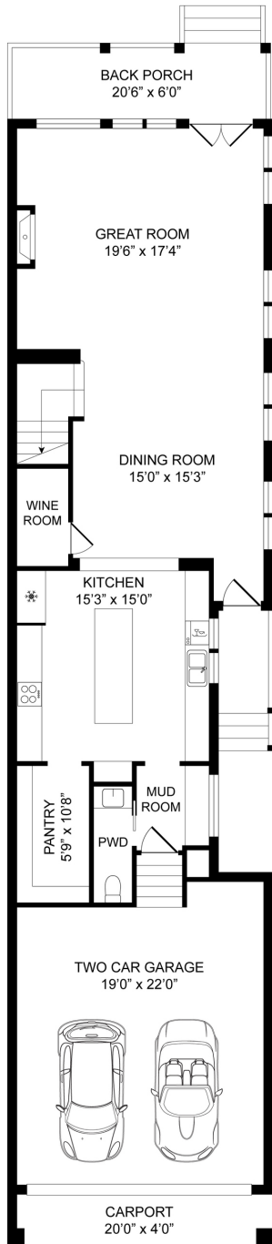
1ST FLOOR
