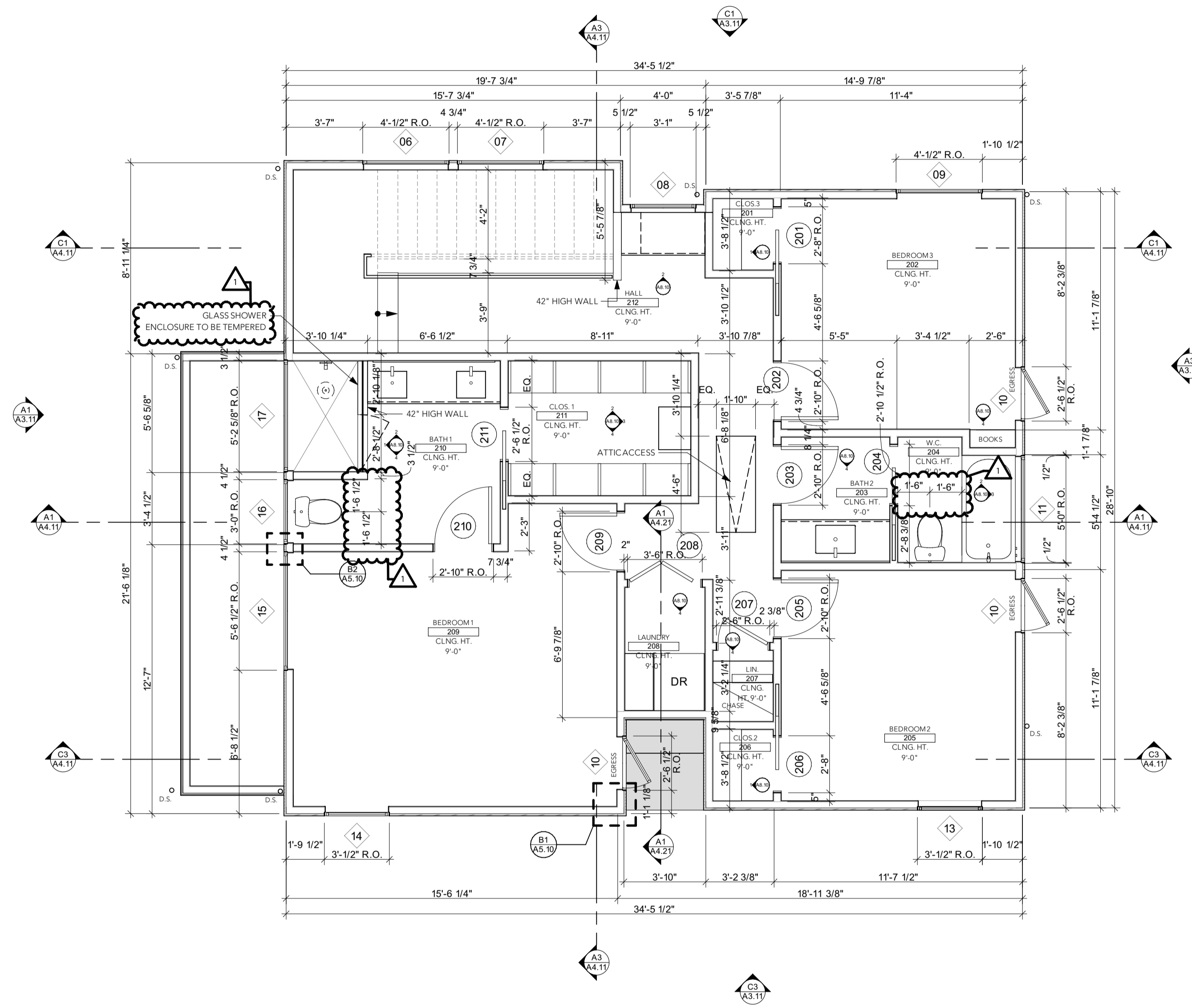
B2 2ND FLOOR PLAN SCALE: 1/4" = 1'-0"
