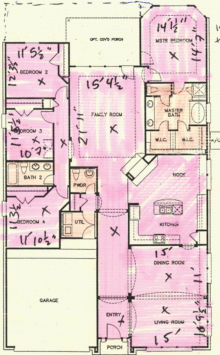
FLOOR PLAN
