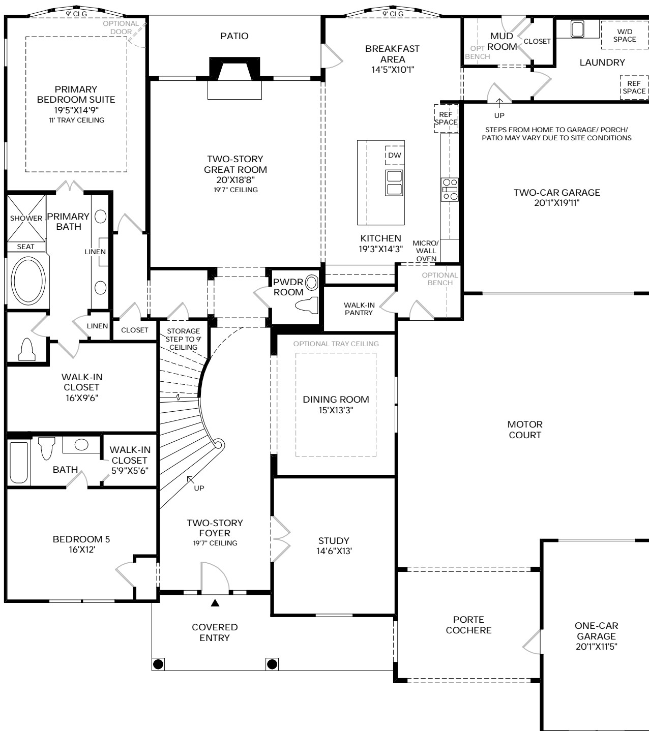
First Floor 10' CEILING HEIGHT
