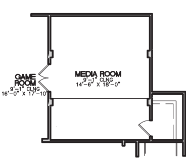
* Media Room Option Second Floor Plan
