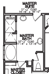
* Baja Shower Option First Floor Plan
