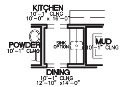
* Butler's Cabinet Option First Floor Plan
