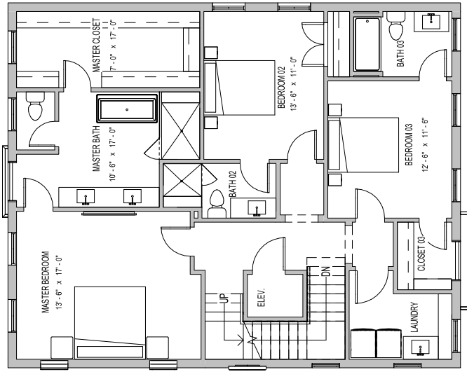
02 SECOND FLOOR PLAN GRAPHIC
