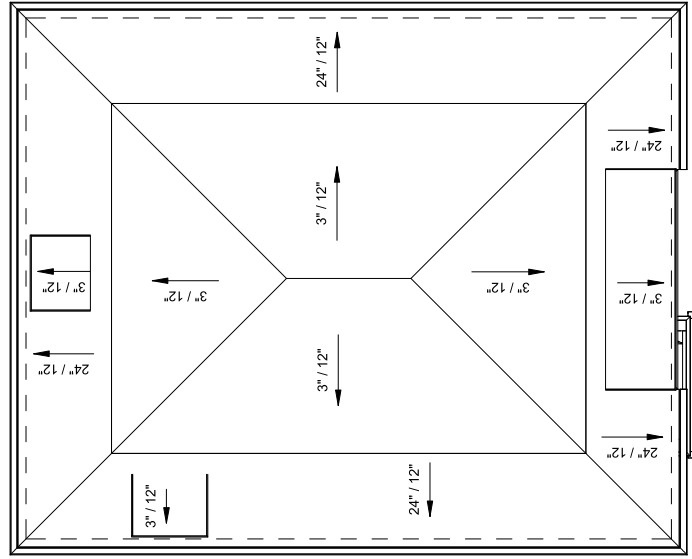
2 ROOF GRAPHIC PLAN SCALE: 1/8" = 1'-0"
