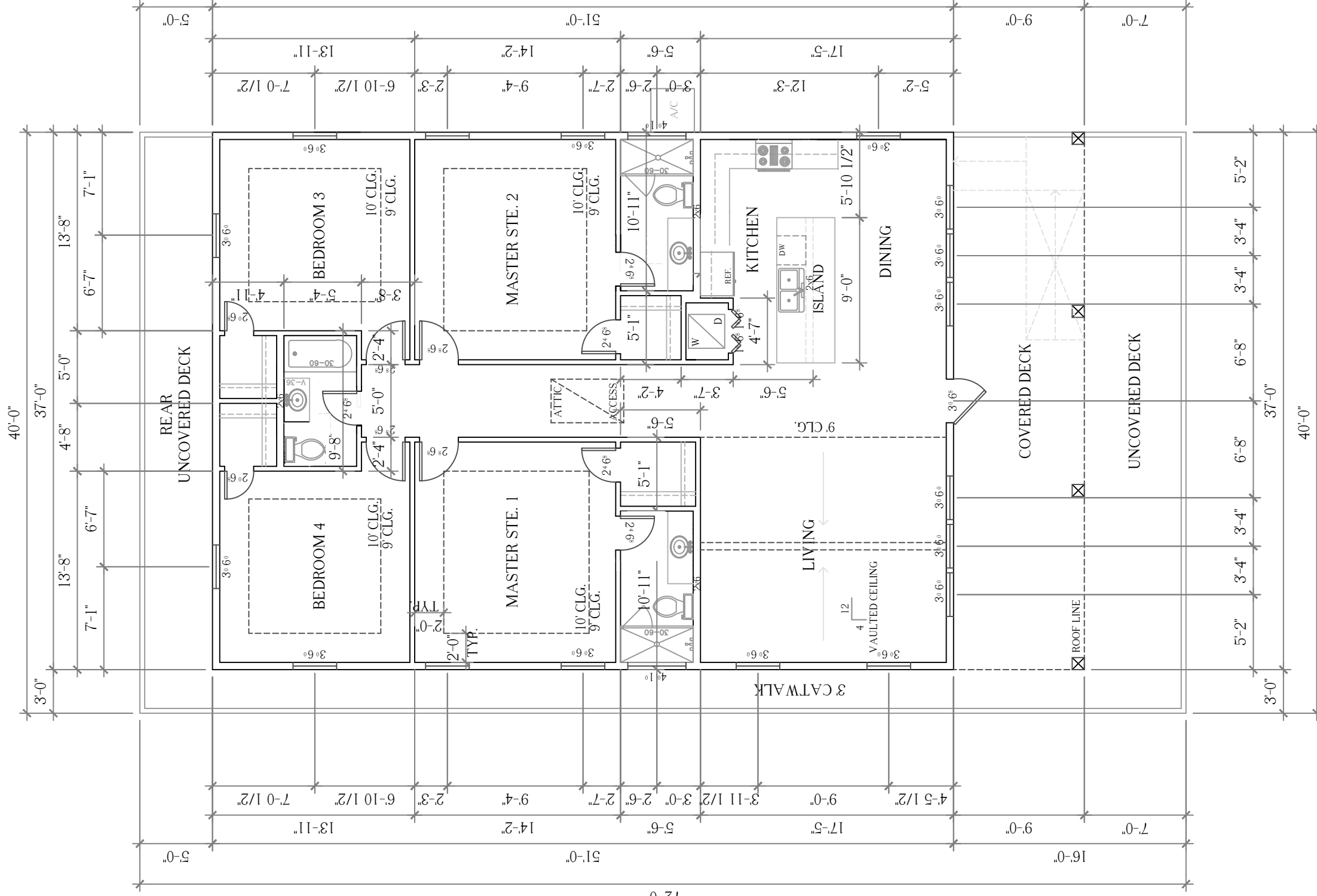
1ST LEVEL FLOOR PLAN
