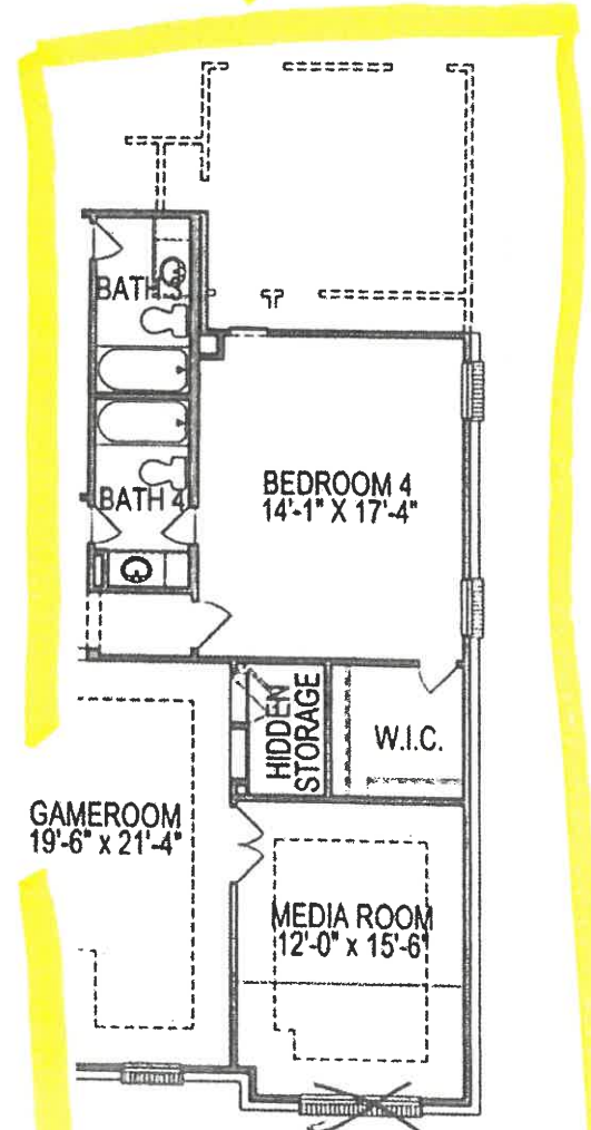
SECOND FLOOR PLAN OPT. #0560 MEDIA ROOM
