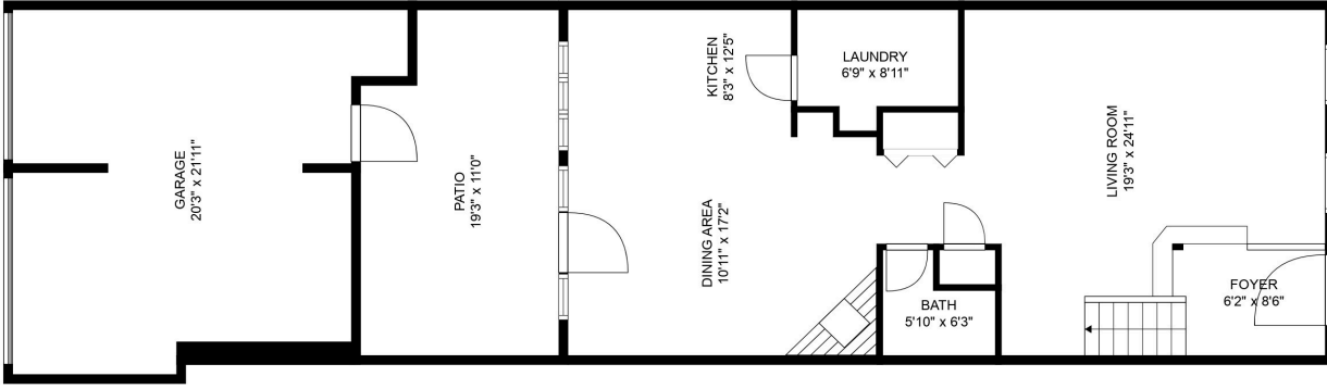
FLOOR 1
