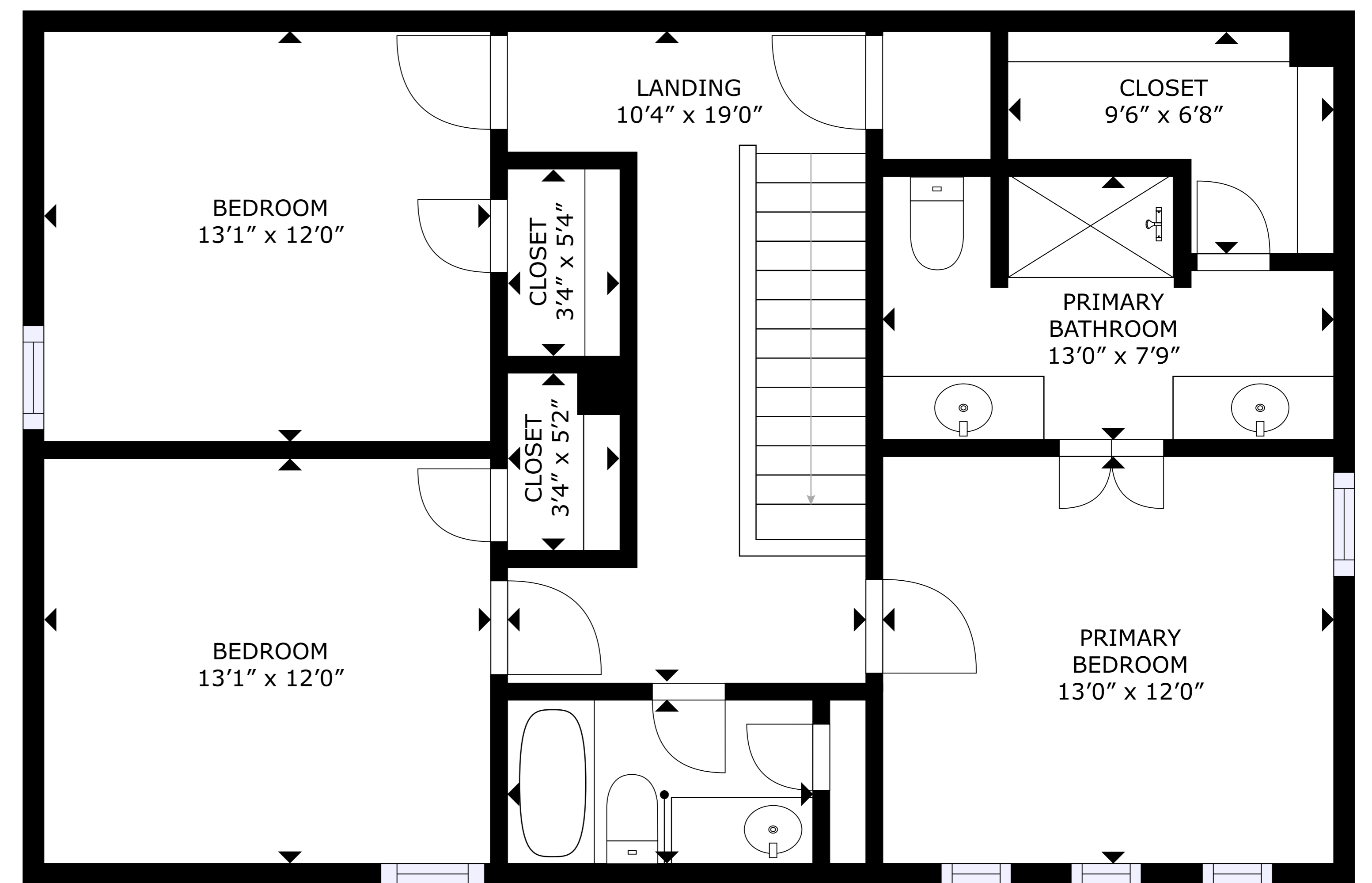
2ND FLOOR
